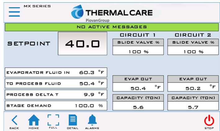
Standard PLC Home Screen
